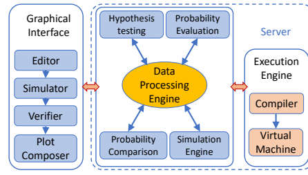
Fig. 2: Architecture of UPPAAL SMC [4]
